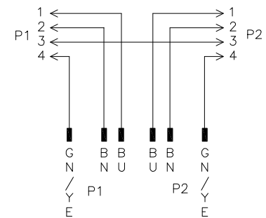
WIRING DIAGRAM
